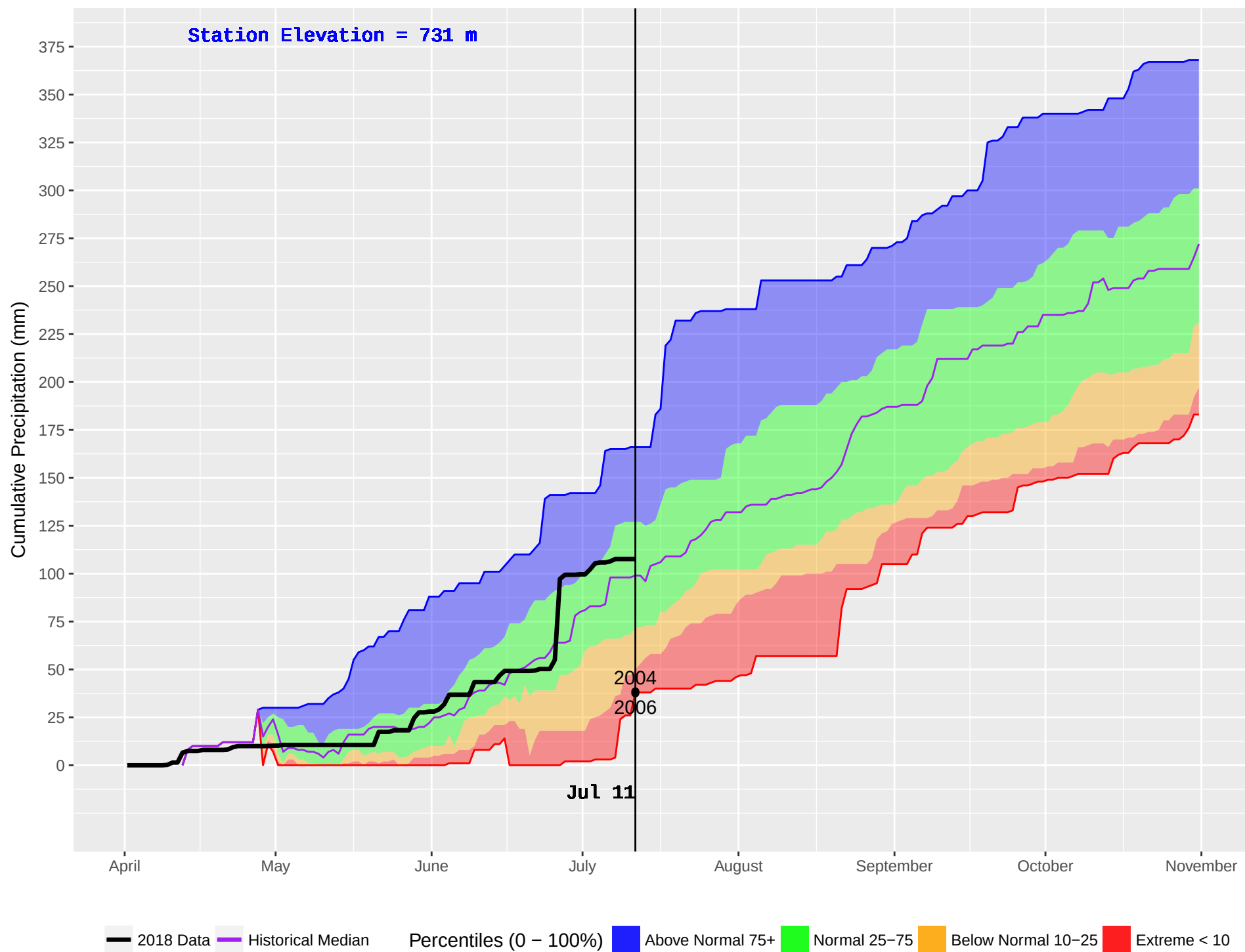
FIRESIDE (440) : Historical (1996–2016) and Current (2018) Noon Cumulative Precipitation
