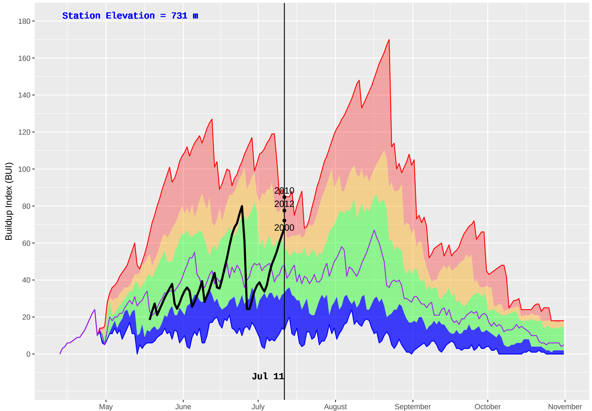
FIRESIDE (440) : Historical (1996–2016) and Current (2018) Noon Buildup Index (BUI)
